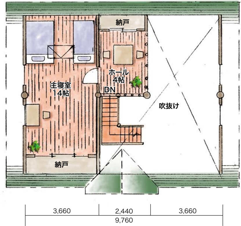
2F PLAN
